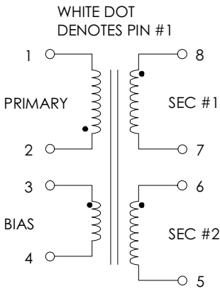
FIGURE 1: SCHEMATIC DIAGRAM
